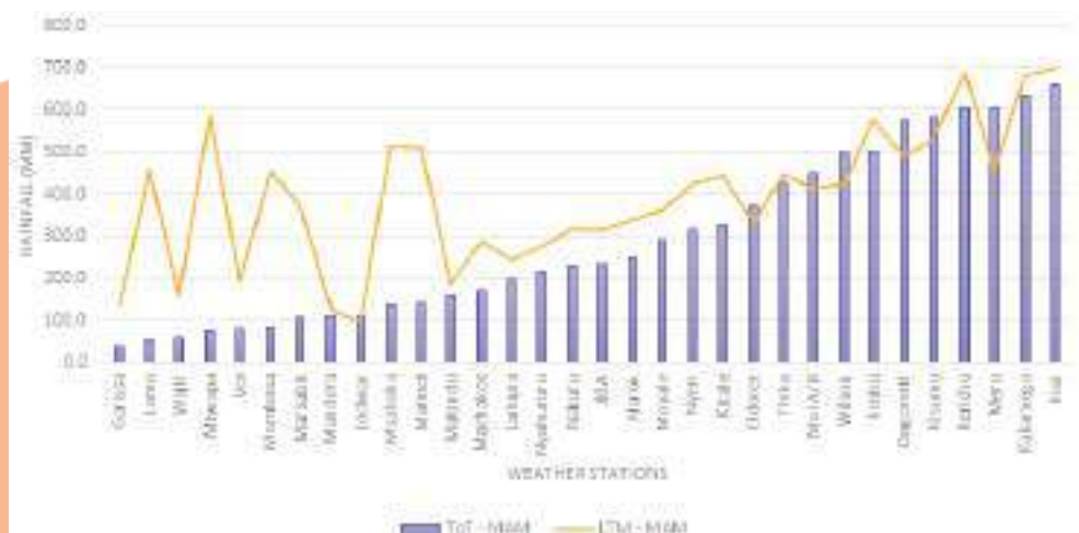
Figure 8.2: Long Rains (March-April-May) Performance, 2021
