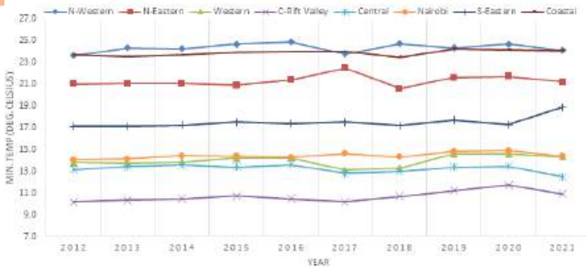
Figure 8.6: Mean Annual Minimum Temperatures, 2012-2021
